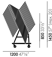
.03 stacking dolly
